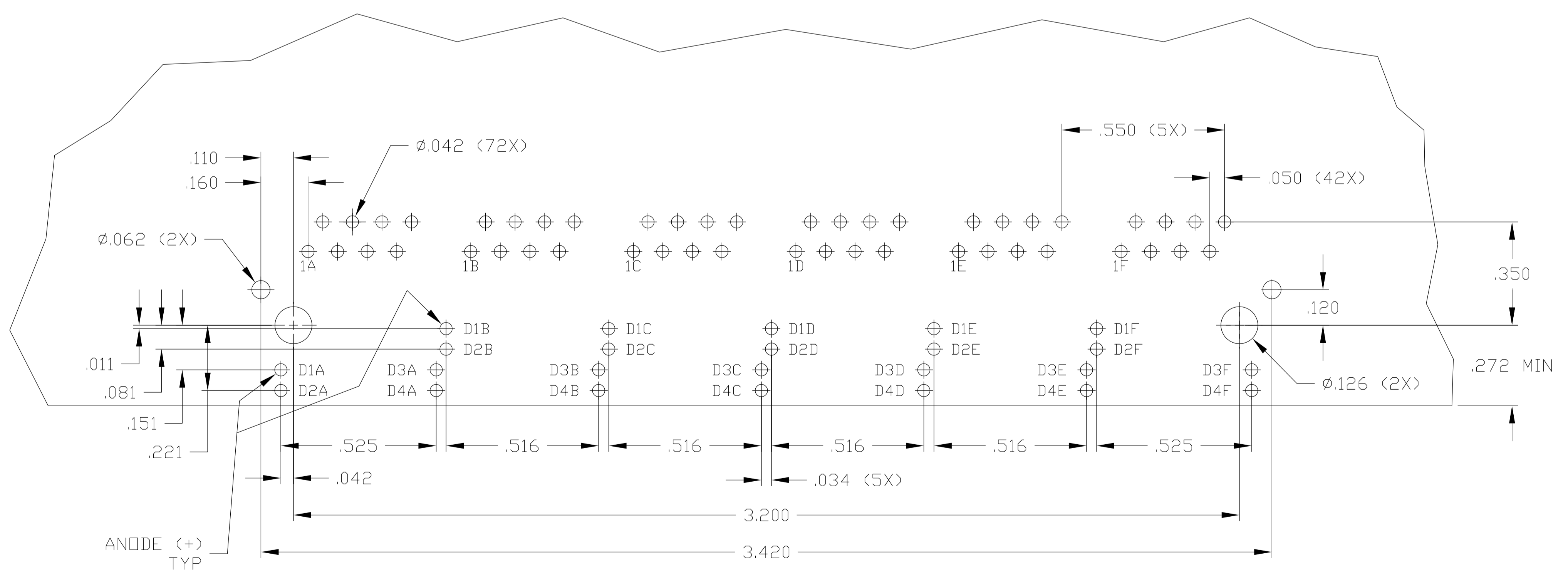
SUGGESTED PCB LAYOUT (Component Side)
